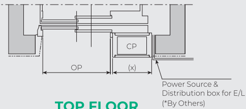
TOP FLOOR
