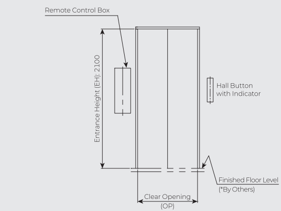
E050 TYPE WITH CP IN HOISTWAY
