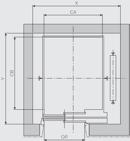
TYPICAL FLOORS
