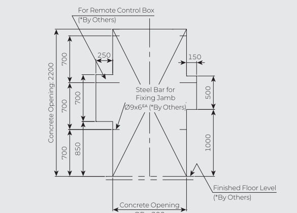
E050 TYPE WITH CP IN HOISTWAY
