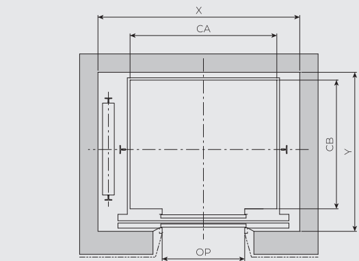
TYPICAL FLOORS
