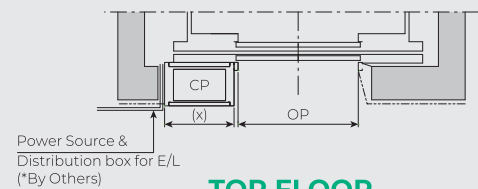
TOP FLOOR
